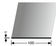
173 U PLATTENSTOß-SCHIENE PANEL RAIL STRIP
