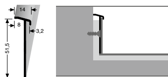
928 FLIESEN SOCKEL TILE BASE
