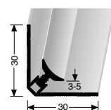
163 U 2-TEILIGE CLIP-INNECKE 2-PART CLIP INTERNAL CORNER
