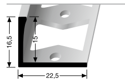
306 G DOPPEL-K PROFILE PERFORATED EDGE TRIM
