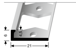
302 G DOPPEL-K PROFILE PERFORATED EDGE TRIM
