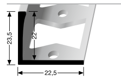
309 G DOPPEL-K PROFILE PERFORATED EDGE TRIM
