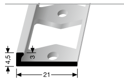
301 G DOPPEL-K PROFILE PERFORATED EDGE TRIM
