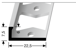
307 G DOPPEL-K PROFILE PERFORATED EDGE TRIM
