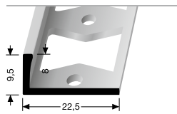
303 G DOPPEL-K PROFILE PERFORATED EDGE TRIM
