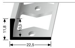
304 G DOPPEL-K PROFILE PERFORATED EDGE TRIM
