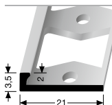
299 G DOPPEL-K PROFILE PERFORATED EDGE TRIM
